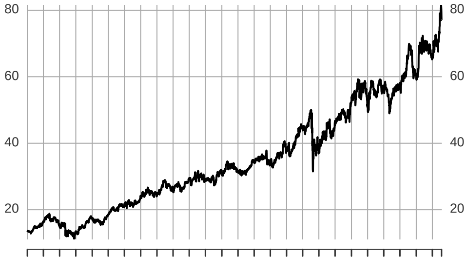
Coca-Cola Closing Stock Price (USD), Adjusted
